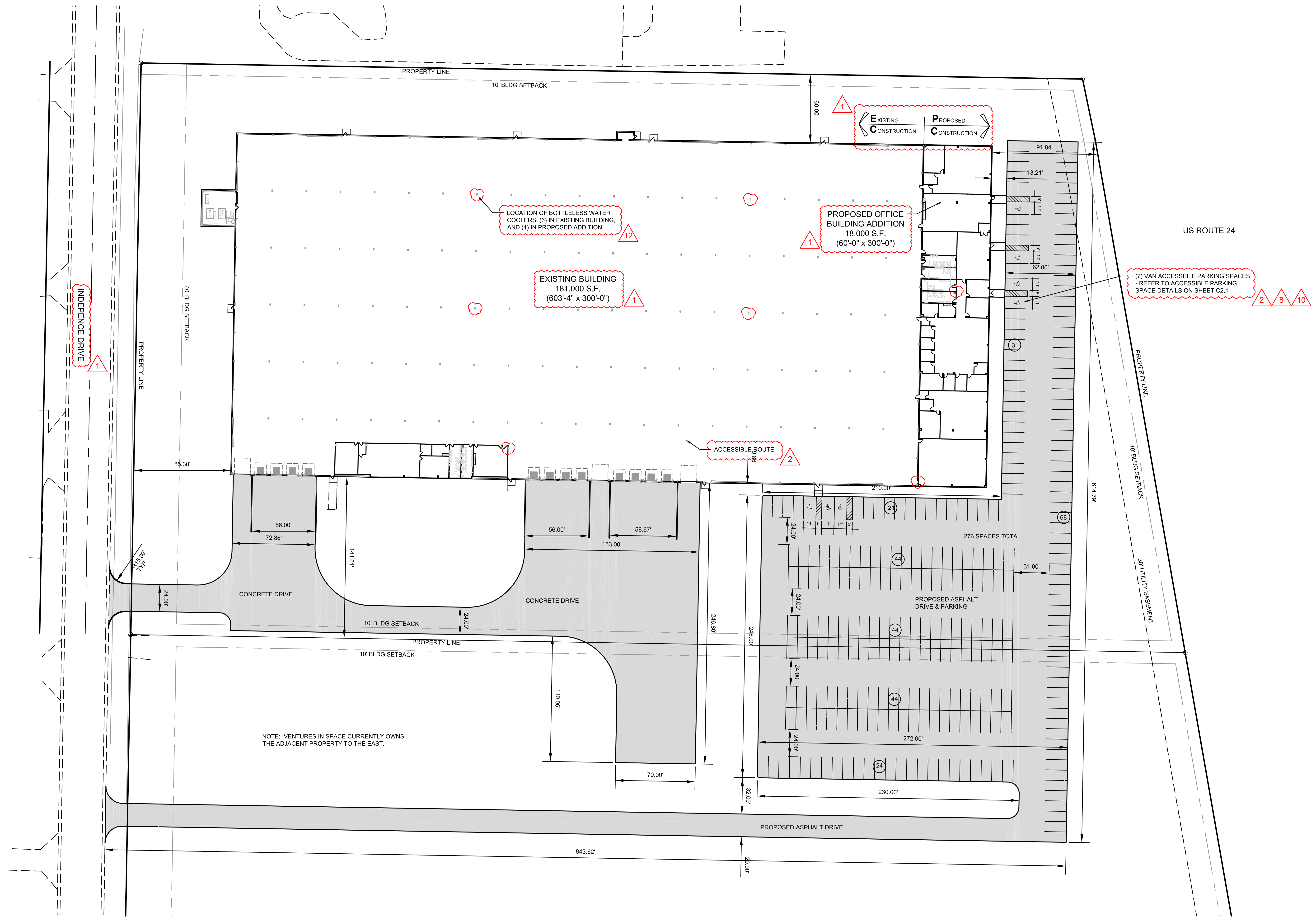
SITE GEOMETRIC PLAN SCALE: 1" = 40'
